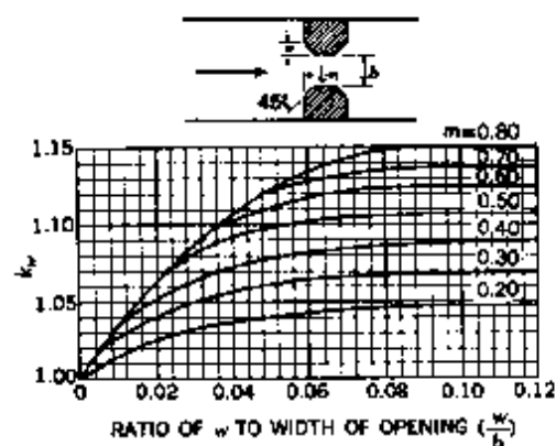
b) 45° wingwalls.
