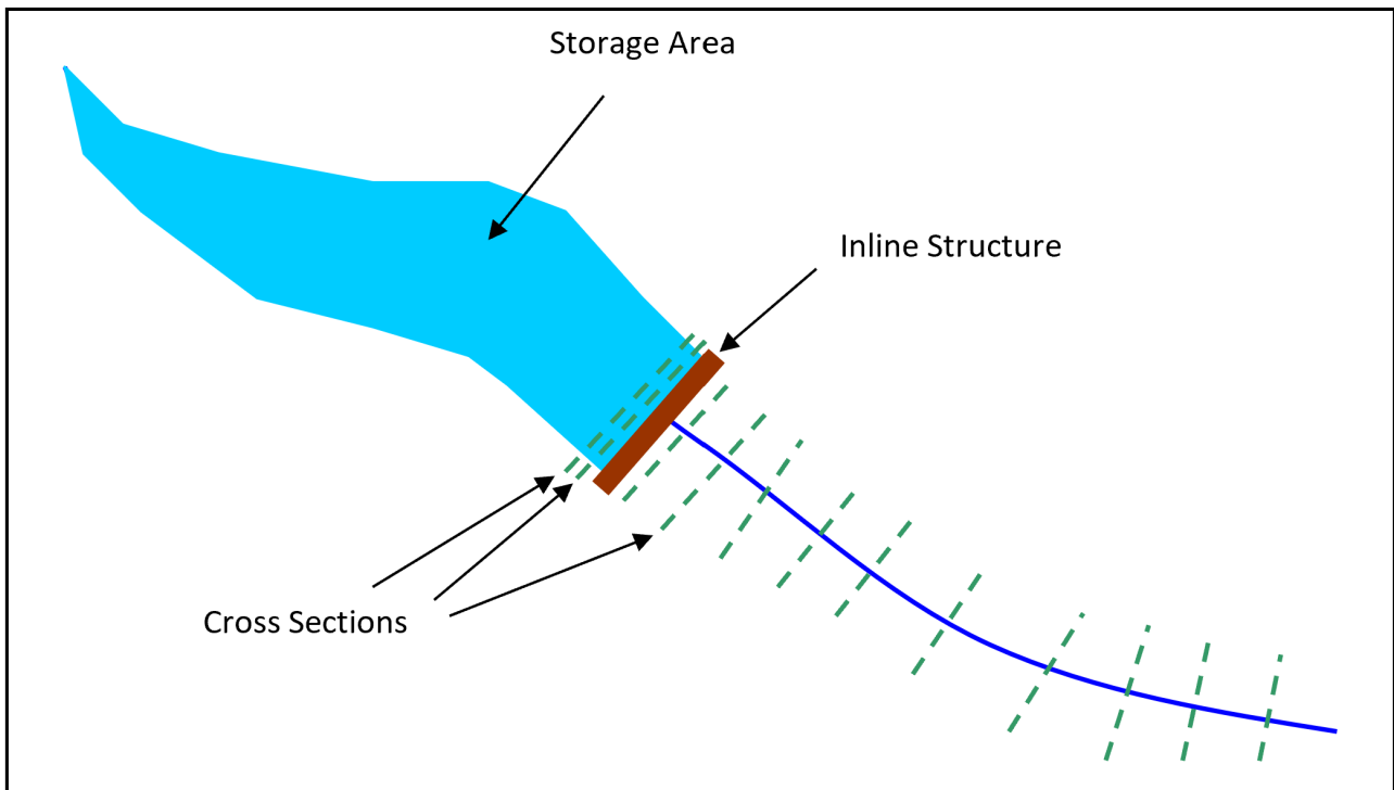
Storage area and cross section layout for level pool routing
