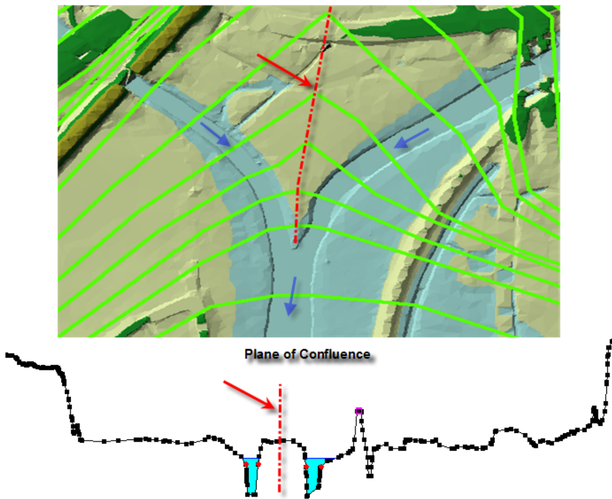
Cross section layout for a tributary coming into a main stem river.
