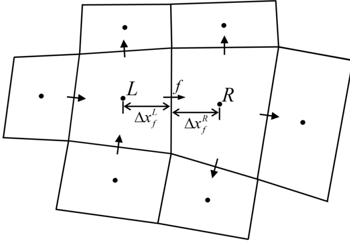
Figure 1. Definition of Eulerian advection variables.
