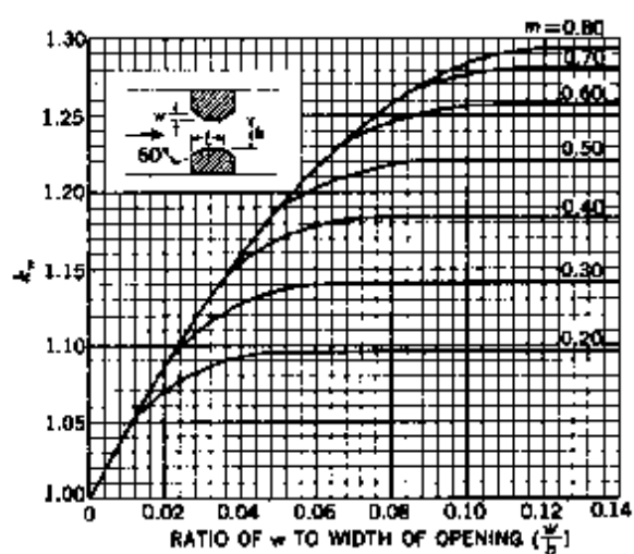
c) 60° wingwalls.
